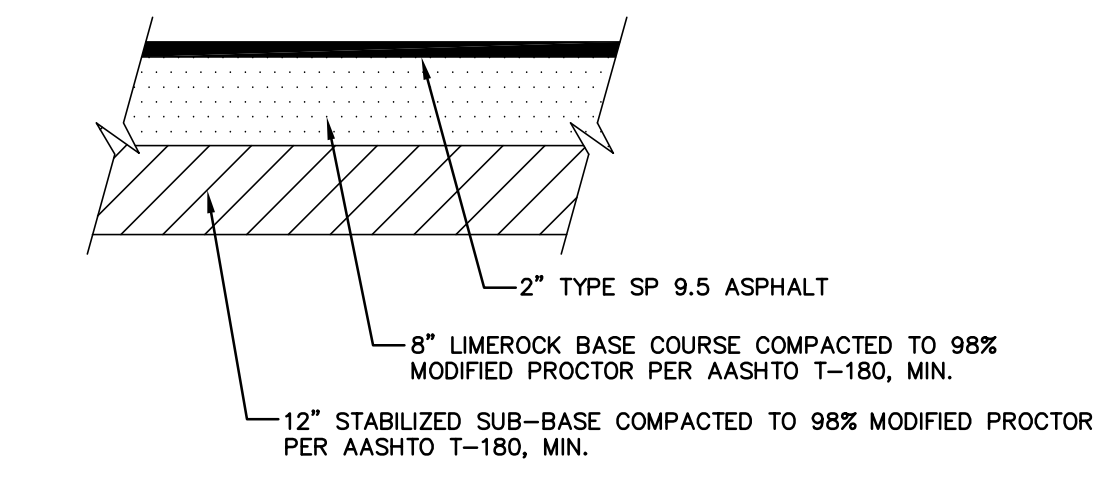
HEAVY DUTY ASPHALT DETAIL N.T.S.
