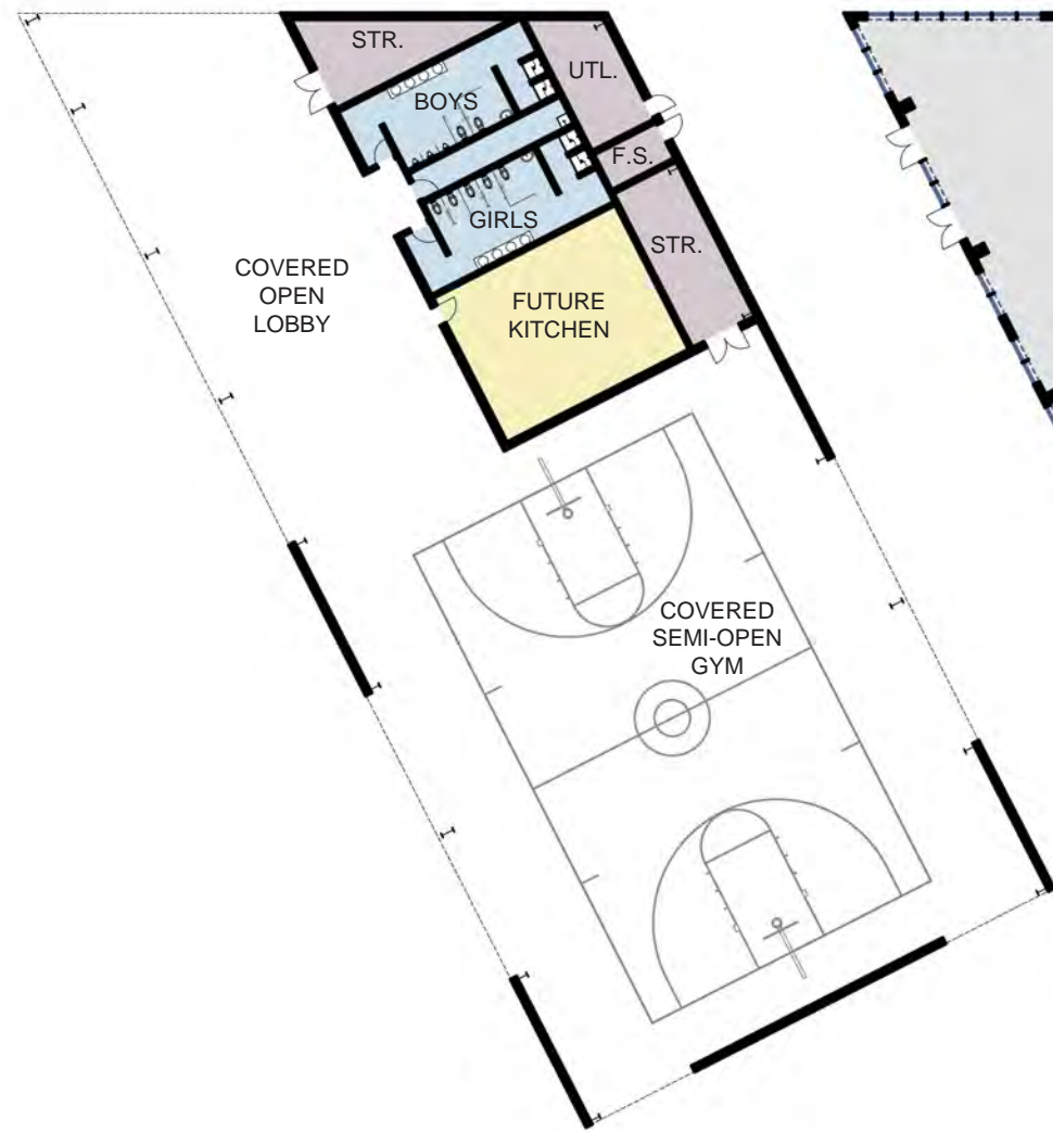
PHASE 1A - 15,000 SQ. FT. SHELL SEMI-ENCLOSED GYM BUILDING
